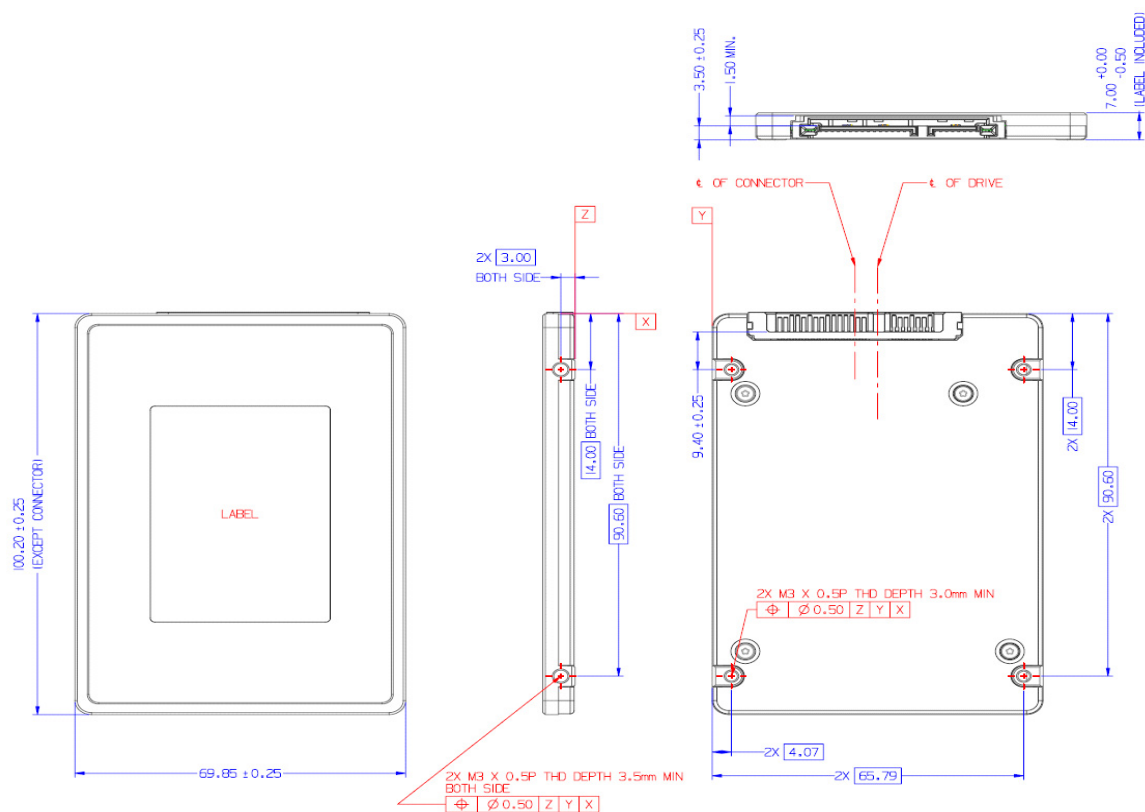
Figure 2. Physical Dimension
