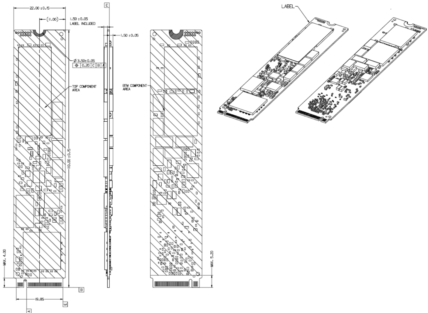
Figure 1. Mechanical Outline
